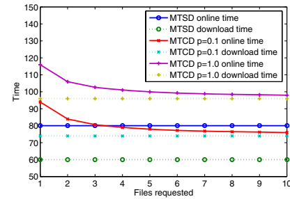
Figure 3. The online time per file and download time per file for peers in different classes in MTCD and MTSD with file correlation of p = 0.1 and p = 1.0 . We assume K = 10 , \mu = 0.02 , \eta = 0.5 , and \gamma = 0.05 for the fluid model.
