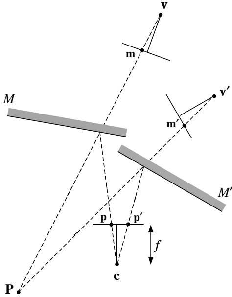
Figure 1: Stereo image formation with a single camera and two planar mirrors. A scene point P reflected off mirrors M and M' is imaged as if seen from two different viewpoints v and v' .
