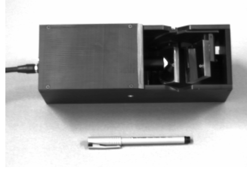
Figure 3: Catadioptric stereo system. By imaging two planar mirrors with a single camera, this compact unit outputs stereo images embedded in a single signal.
