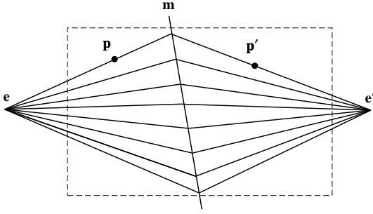
Figure 2: The epipolar geometry of planar motion. When motion is constrained to lie in a plane, all corresponding epipolar lines must intersect at m the image of the axis of rotation. Therefore, the two epipoles e and e' and the line m completely determine the epipolar geometry.
