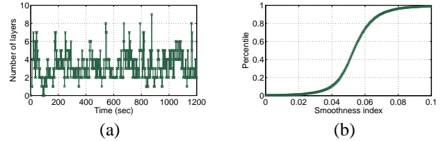
Fig. 13. Video quality of free-riders. (a) Behavior of typical free-riders; (b) Cumulative distribution of smoothness index.
