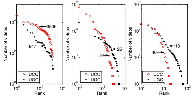
Figure 8: UCC uploaders vs. UGC uploaders in terms of number of uploaded videos. (a) Popular uploaders; (b) Social uploaders; (c) Random uploaders.
