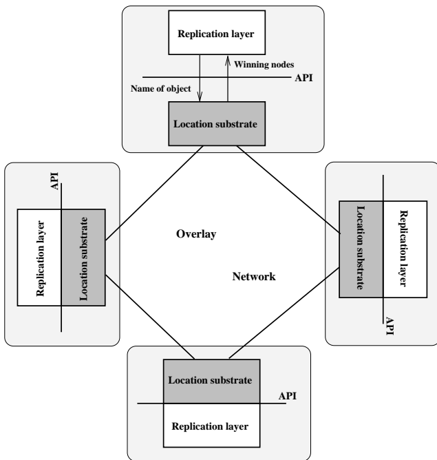
Figure 2: API
